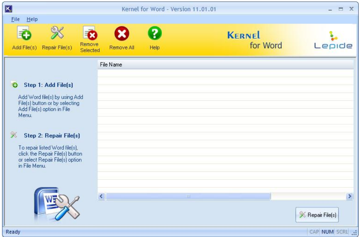
Figure 3.2.1 Main Window
