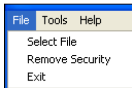
Figure 3.1: File Menu
